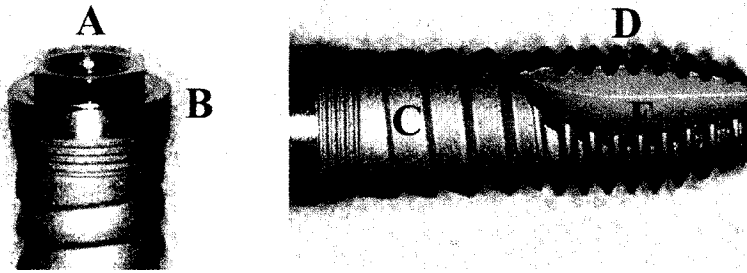
FIGURE 1. The study implant: (A) standard external hex, (B) polished 0.7-mm titanium collar, (C) 6.5-mm with stress-diversion thread, (D) tapered self-tapping implant body, (E) cutout in the driving thread.
